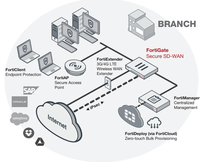
FortiGate 600E deployment in branch office (Secure SD-WAN)
